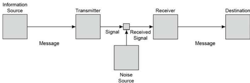
VISUALIZATION OF THE COMMUNICATION MODEL AS OUTLINED BY SHANNON AND WEAVER.
